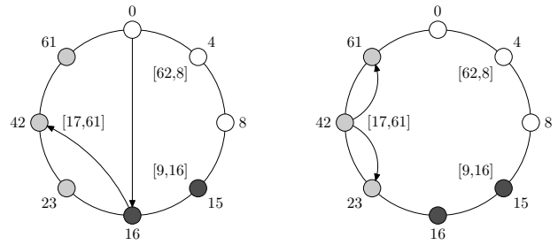
Step 1: find neighborhood Step 2: broadcast Figure 1: Penny message propagation
