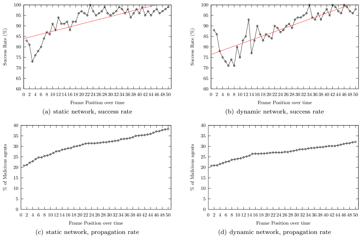
Figure 12: RDF malware propagation experiment success and propagation rates
